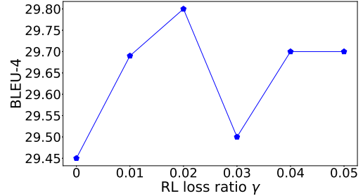
Fig. 3: Effect of RL ratio for G2S+AE+RL on WQ.
