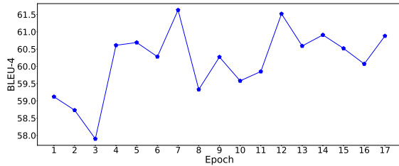
Fig. 6: Convergence analysis for G2S+AE on PQ.
