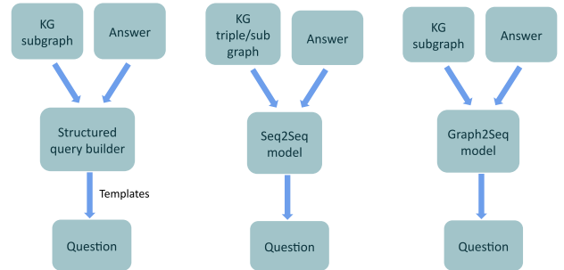
Fig. 1: Various QG from KGs learning paradigms. Left: template-based approaches. Middle: Seq2Seq-based approaches for simple QG from a single KG triple or multi-hop QG from a KG subgraph. Right (ours): Graph2Seq-based approaches for multi-hop QG from a KG subgraph.
