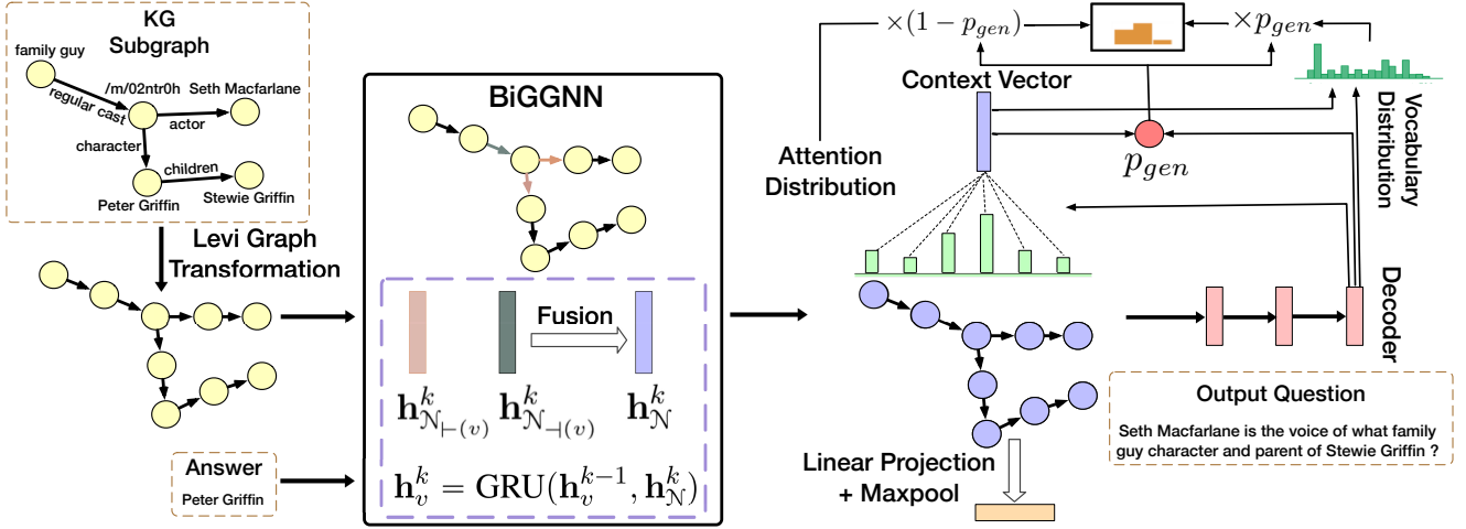
Fig. 2: Overall architecture of our proposed model. Best viewed in color.
