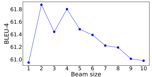
Fig. 5: Effect of beam search size for G2S+AE on PQ.
