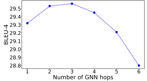
Fig. 4: Effect of number of GNN hops for G2S+AE on WQ.
